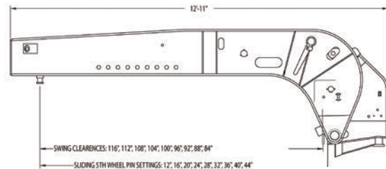
XL CHEATER GOOSENECK 12' 11" OAL
