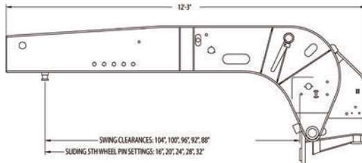
XL CHEATER GOOSENECK 12' 3" OAL
